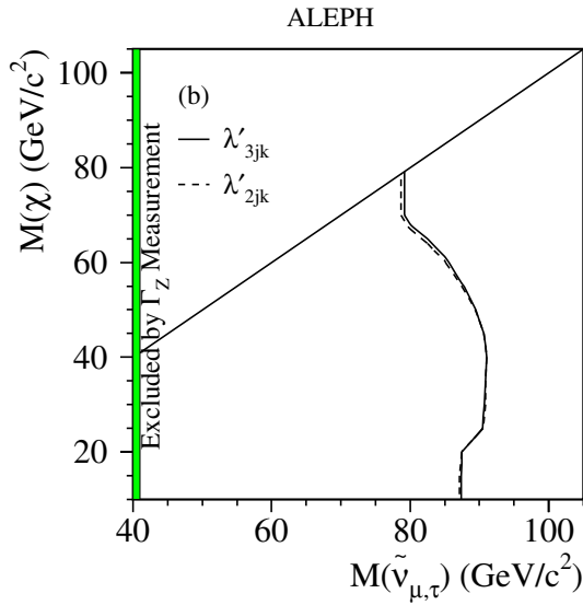
Fig. 11. The 95% C.L. limits in the (m_\chi, m_{\tilde{\nu}}) plane for a electron and b muon or tau sneutrinos decaying indirectly via a dominant LQ\bar{D} operator. The two choices of \lambda'_{2jk} and \lambda'_{3jk} correspond to the most and least stringent exclusions, respectively. The electron sneutrino cross section is evaluated at \mu = -200 \text{ GeV}/c^2 and \tan \beta = 2
