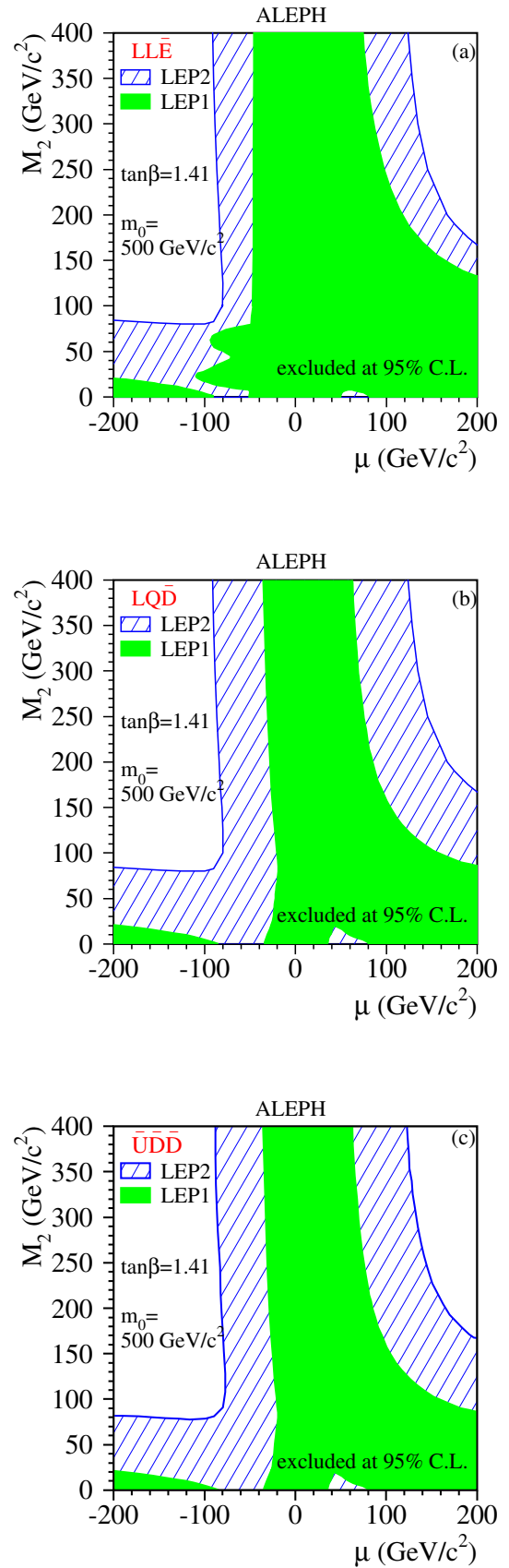
Fig. 3a–c. Regions in the (\mu, M_2) plane excluded at 95% C.L. at \tan\beta = 1.41 and m_0 = 500 \text{ GeV}/c^2 for the three operators a \lambda , b \lambda' and c \lambda'' .
