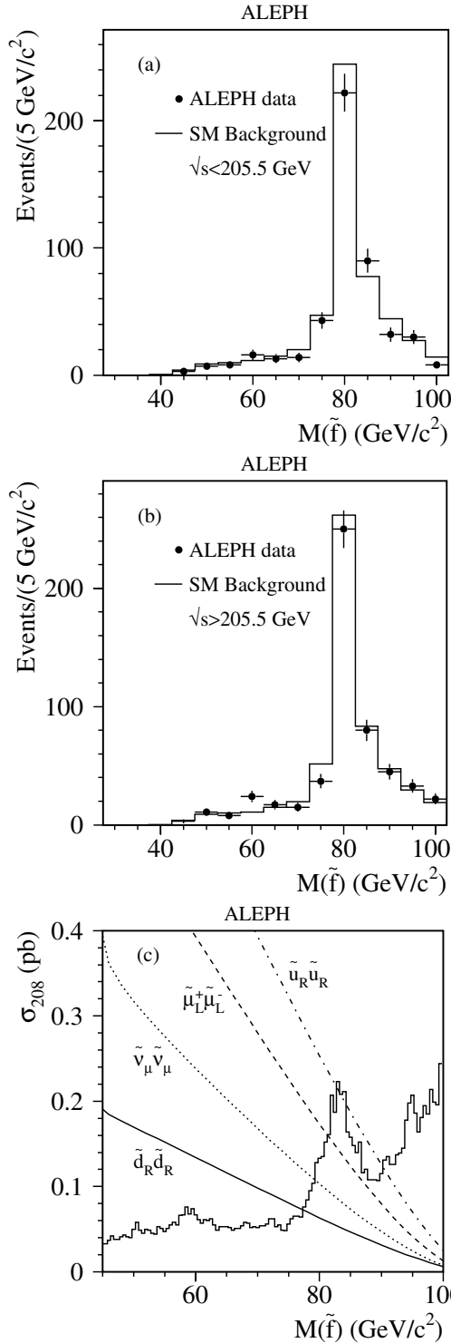
Fig. 9a–c. The distributions of the reconstructed jet-pair invariant masses after forcing each event into four jets. The points are the data taken in year 2000, for a the 205 GeV sample and b the 207 GeV sample. The solid histogram is the predicted Standard Model background. In c , the 95% C.L. cross section upper limit for sleptons (via LQ\bar{D} ), sneutrinos (via LQ\bar{D} ) and squarks (via \bar{U}\bar{D}\bar{D} ) decaying directly to four jets is shown. The MSSM cross sections for pair production of muon sneutrinos, left-handed smuons and right-handed squarks are superimposed
