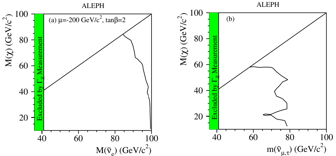
Fig. 14. a The 95% C.L. limits in the (m_\chi, m_{\tilde{\nu}_e}) plane for \tilde{\nu}_e decaying indirectly via a dominant \bar{U}\bar{D}\bar{D} operator. The \tilde{\nu}_e cross section is evaluated at \mu = -200 \text{ GeV}/c^2 and \tan\beta = 2 . b The exclusion obtained in the (m_\chi, m_{\tilde{\nu}_{\mu,\tau}}) plane for \tilde{\nu}_{\mu,\tau} decaying indirectly via a dominant \bar{U}\bar{D}\bar{D} operator
