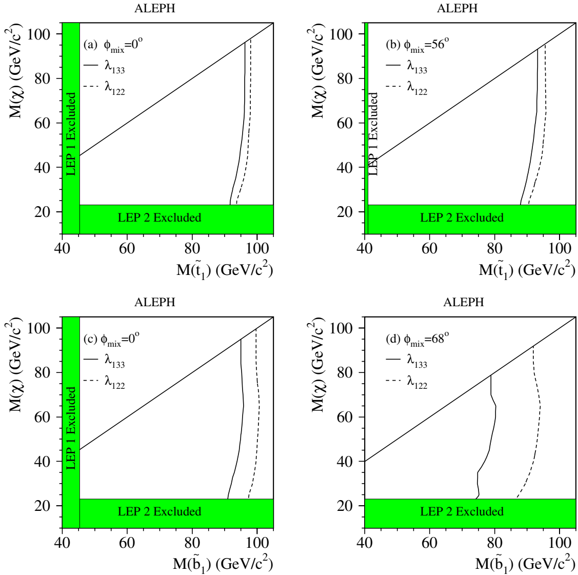
Fig. 4a–d. The 95% C.L. limits in a,b the (m_\chi, m_{\tilde{t}_1}) plane and c,d the (m_\chi, m_{\tilde{b}_1}) plane for indirect decays via the LL\bar{E} couplings \lambda_{122} and \lambda_{133} , for no mixing ( \phi_{\text{mix}} = 0^\circ ) and for \phi_{\text{mix}} = 56^\circ and 68^\circ , corresponding to vanishing coupling to the Z, for stops and sbottoms, respectively. The LEP 2 exclusion corresponds to the absolute limit on m_\chi
