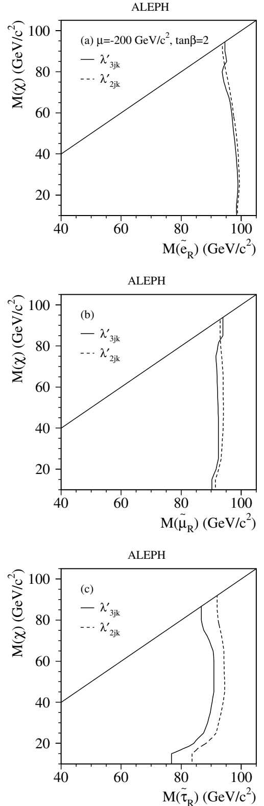
Fig. 10a–c. The 95% C.L. limits in the (m_\chi, m_{\tilde{\ell}_R}) plane for a selectrons, b smuons and c staus decaying indirectly via a dominant LQ\bar{D} operator. The two choices of \lambda'_{2jk} and \lambda'_{3jk} correspond to the most and least stringent exclusions, respectively. The selectron cross section is evaluated at \mu = -200 \text{ GeV}/c^2 and \tan\beta = 2 . The limit from the \Gamma_Z measurements excludes m_{\tilde{\ell}} < 38 \text{ GeV}/c^2
