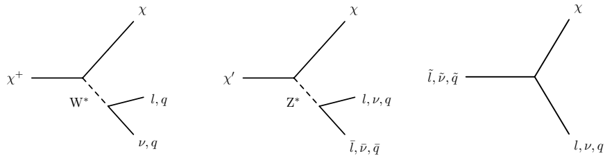
Fig. 2. Indirect decays of supersymmetric particles. The neutralino \chi decays directly via the \lambda , \lambda' and \lambda'' couplings as illustrated in Fig. 1
