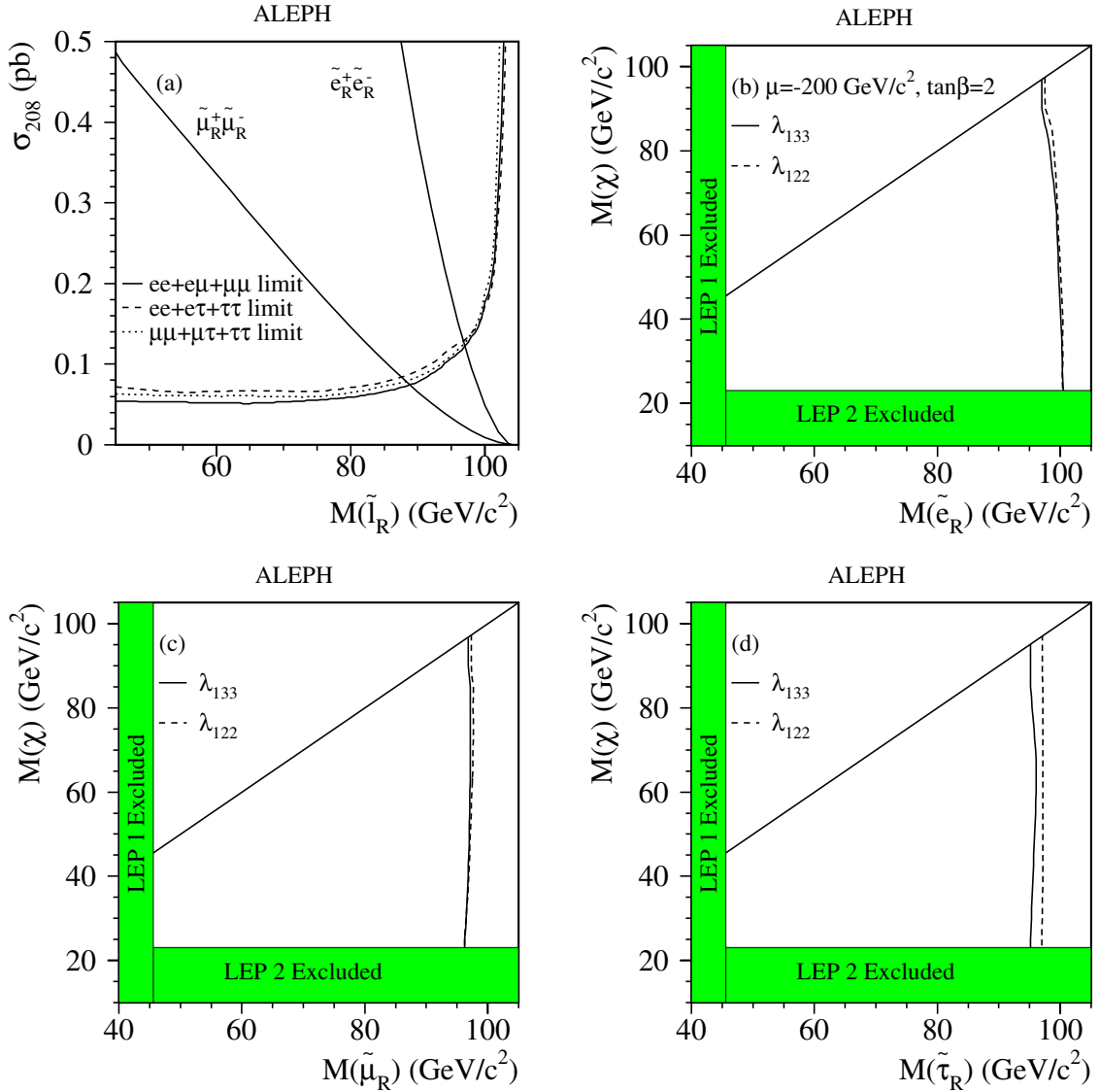
Fig. 5. a The 95% C.L. cross section upper limits for sleptons decaying directly via a dominant LL\bar{E} operator. The MSSM cross sections for pair production of right-handed selectrons and smuons are superimposed. The 95% C.L. limits in the (m_\chi, m_{\tilde{e}_R}) plane for indirect decays of selectrons b , smuons c and staus d . The two choices of \lambda_{122} and \lambda_{133} correspond to the most and least stringent exclusions, respectively. The selectron cross section is evaluated at \mu = -200 \text{ GeV}/c^2 and \tan\beta = 2
