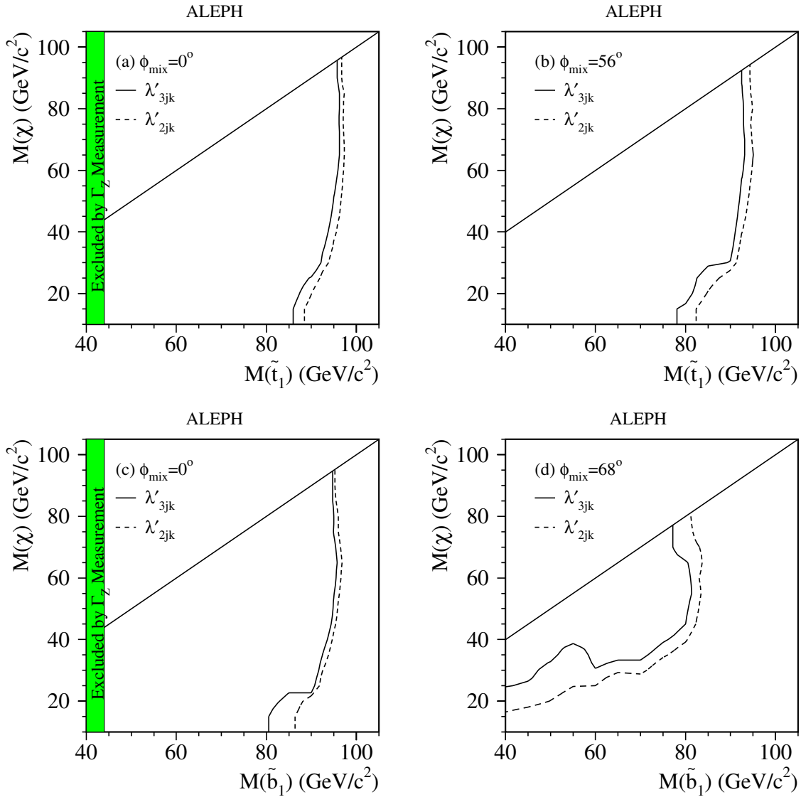
Fig. 8. The 95% C.L. limits in a,b the (m_\chi, m_{\tilde{t}_1}) plane and c,d the (m_\chi, m_{\tilde{b}_1}) plane for indirect decays via a \lambda'_{211} or \lambda'_{311} LQ\bar{D} coupling, for no mixing ( \phi_{\text{mix}} = 0^\circ ) and for \phi_{\text{mix}} = 56^\circ and 68^\circ for stops and sbottoms, respectively
