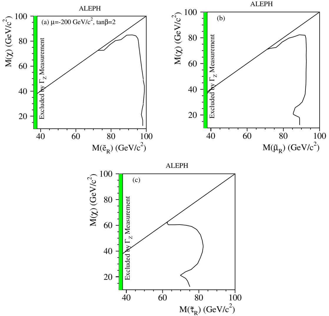
Fig. 13. The 95% C.L. limits in the (m_\chi, m_{\tilde{l}}) plane for a selectrons, b smuons and c staus decaying indirectly via a dominant \bar{U}\bar{D}\bar{D} operator. The selectron cross section is evaluated at \mu = -200 \text{ GeV}/c^2 and \tan\beta = 2
