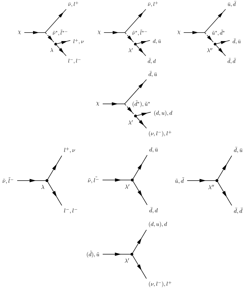
Fig. 1. Direct R-parity violating decays of supersymmetric particles via the \lambda , \lambda' and \lambda'' couplings. The points mark the R-parity violating vertex in the decay
