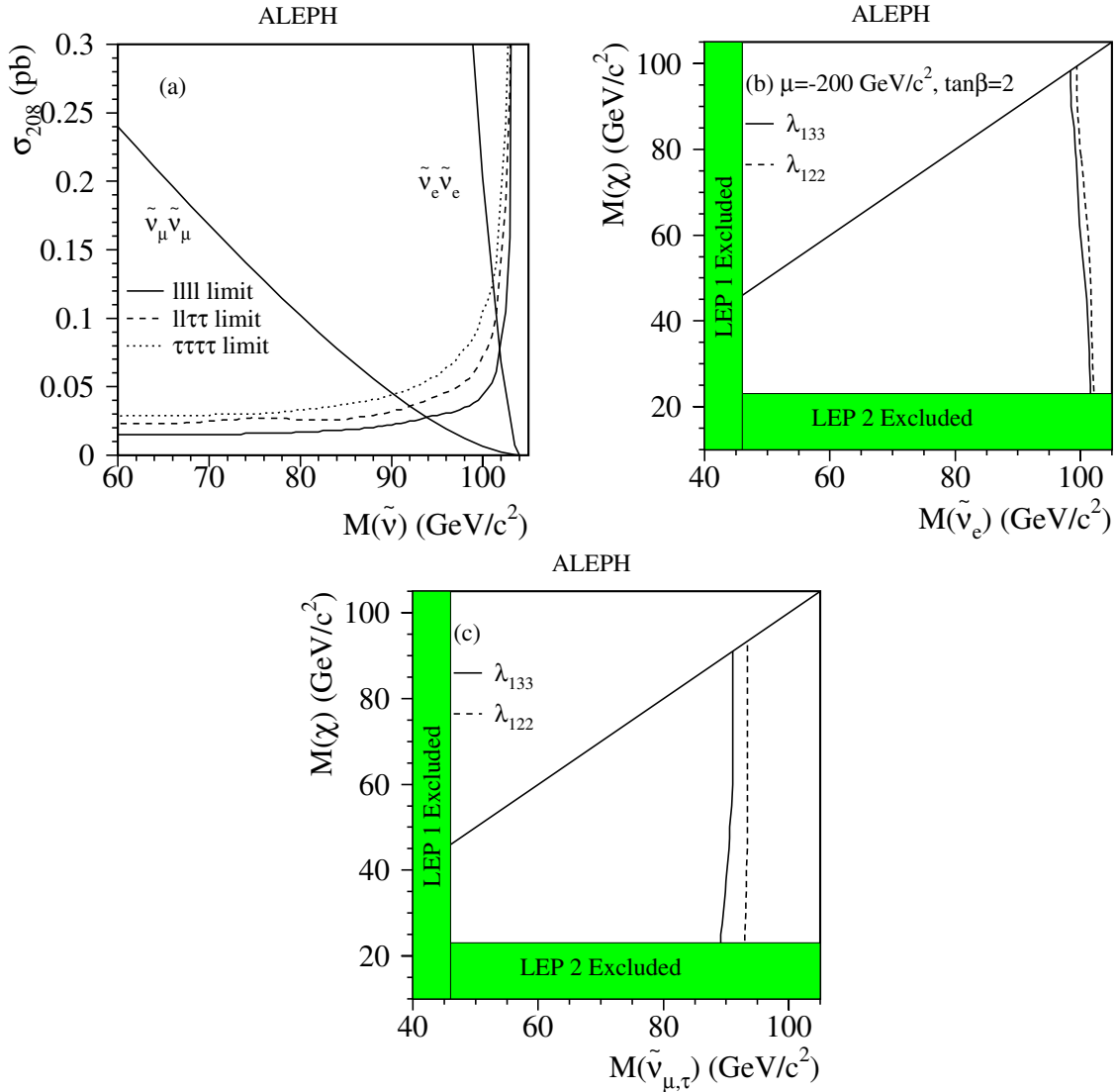
Fig. 6. a The 95% C.L. cross section upper limits for sneutrinos decaying directly via a dominant LL\bar{E} operator. The three curves correspond to different possible final states, with \ell = e or \mu , due to the specific choice of sneutrino flavour and \lambda_{ijk} . The MSSM cross section for pair production of muon and electron sneutrinos are superimposed; the tau sneutrinos have the same cross section as the muon type. The 95% C.L. limits in the (m_\chi, m_{\tilde{\nu}}) plane for \tilde{\nu}_e b and for both \tilde{\nu}_\mu and \tilde{\nu}_\tau c indirect decays. The two choices of \lambda_{122} and \lambda_{133} correspond to the most and least stringent exclusions, respectively. The electron sneutrino cross section is evaluated at \mu = -200 \text{ GeV}/c^2 and \tan\beta = 2
