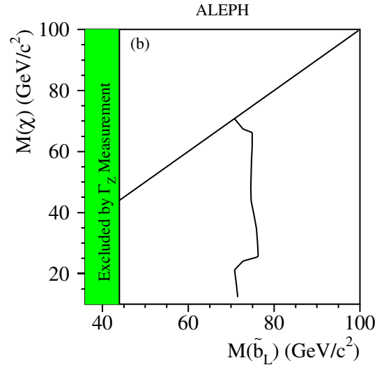
Fig. 12. The 95% C.L. limits in a the (m_\chi, m_{\tilde{t}_L}) plane and b the (m_\chi, m_{\tilde{b}_L}) plane for indirect decays via the \bar{U}\bar{D}\bar{D} couplings
