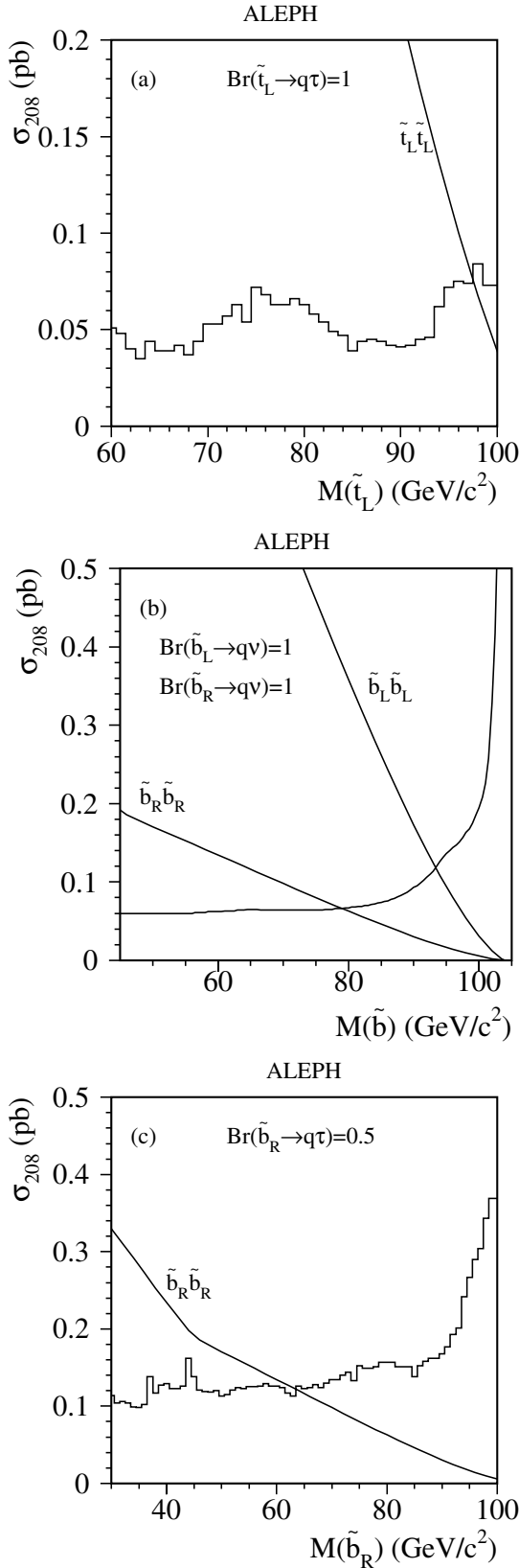
Fig. 7a–c. The 95% C.L. cross section upper limits for the production of squarks decaying directly via a dominant LQ\bar{D} operator: the limits are shown for \tilde{t}_L ( \lambda'_{33k} ), \tilde{b}_L ( \lambda'_{i3k} ) or \tilde{b}_R ( \lambda'_{i33} ), and \tilde{b}_R ( \lambda'_{3j3} ) in a , b and c , respectively. The expected MSSM cross sections are superimposed
